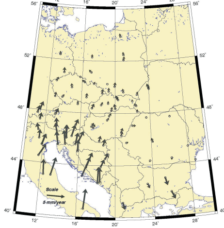
Fig. 4: Estimated horizontal velocity field from combination of epoch-wise and permanent networks.
